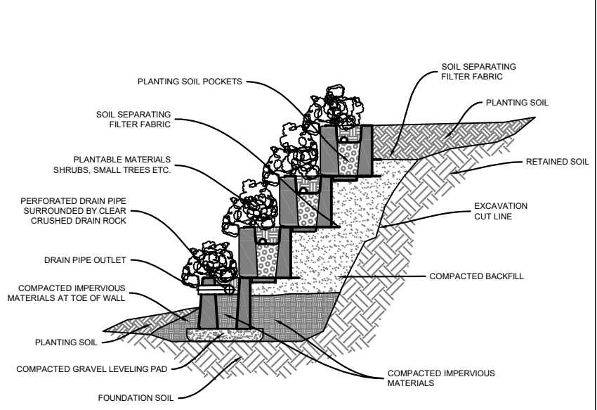
2.0 FT PLANTABLE WALL
