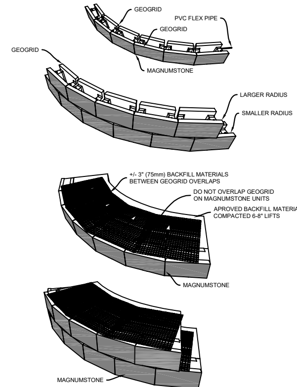
OUTSIDE CURVE
