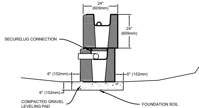
LEVELING PAD
