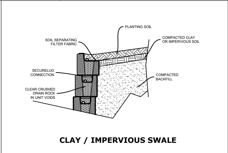
4.0 FT PLANTABLE WALL
