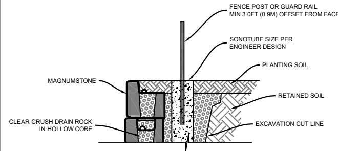
GUARD RAIL
