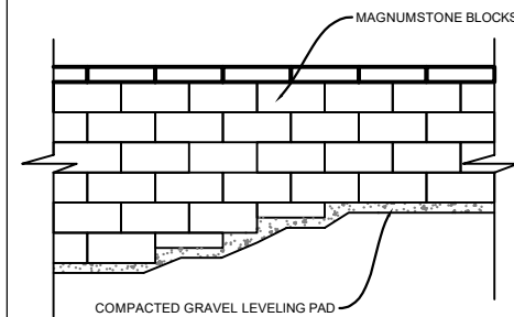
BASE STEP UP
