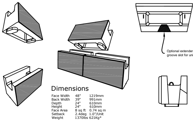
STANDARD UNIT
