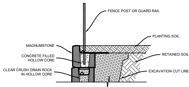
FENCE THROUGH HOLLOW CORE
