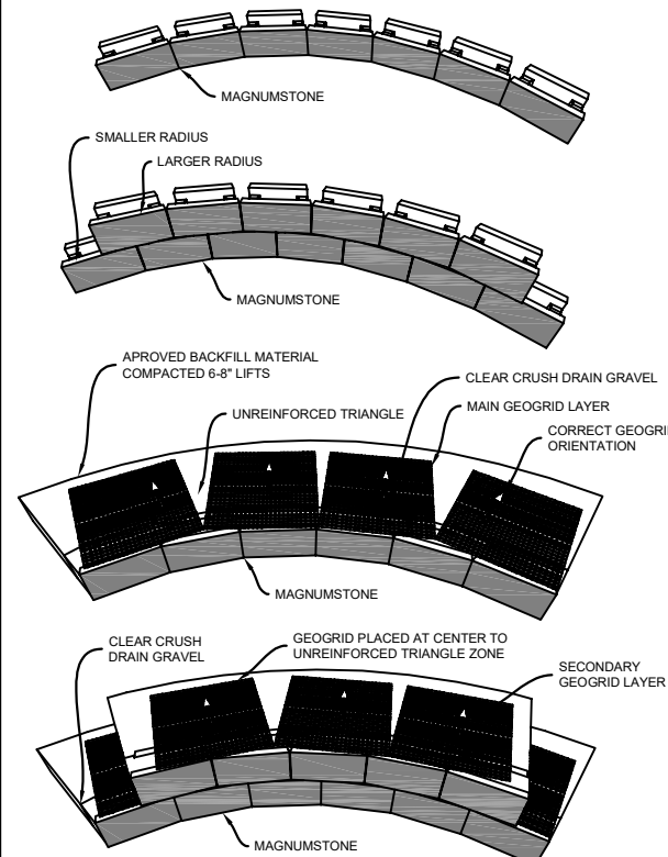
INSIDE CURVE
