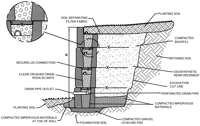
STANDARD UNIT
