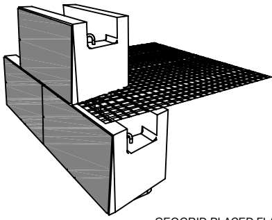
GEOGRID PLACED FLAT AND TAUGHT FOR MAXIMUM SECURE LUG CONNECTION
