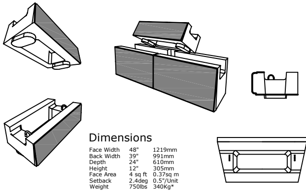
HALF HIGH UNIT
