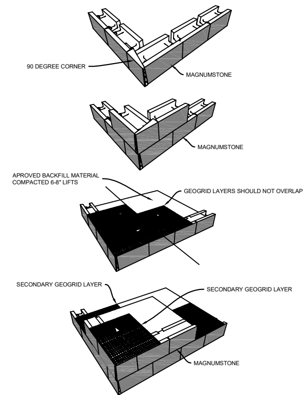
OUTSIDE CORNER
