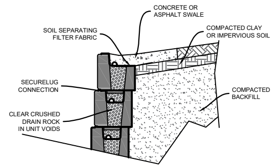
CONCRETE / ASPHALT SWALE
