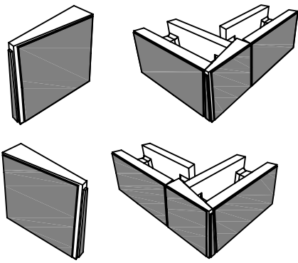
CORNER/END UNIT
