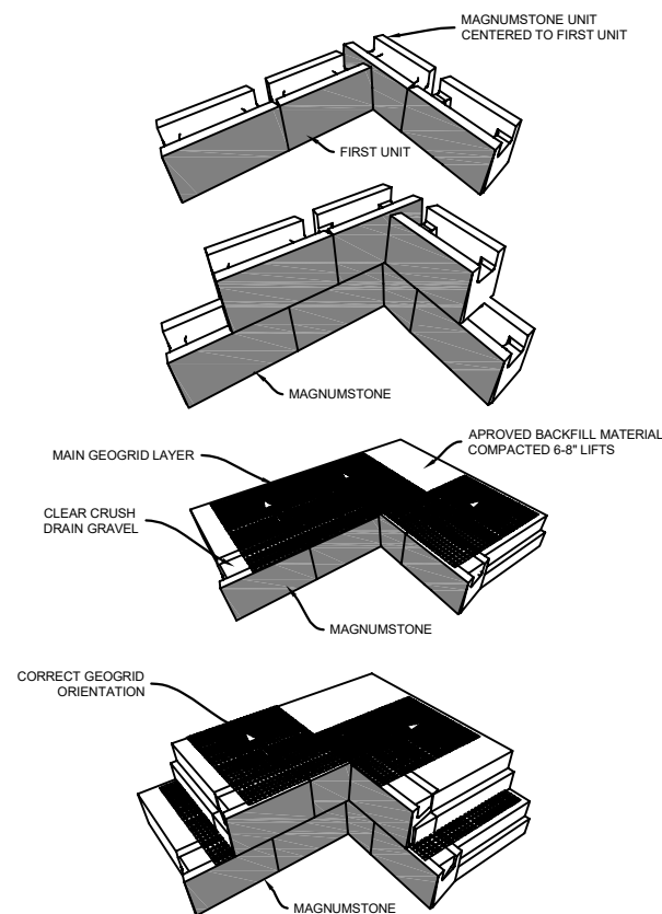
INSIDE CORNER
